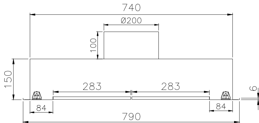
Vista Frontal
